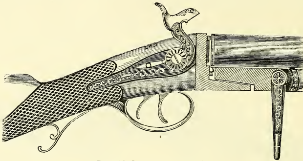
Dougall's Lock-fast Breech-action.
